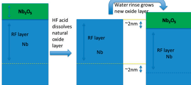
Figure 1: Schematic of the principle behind HF/water rinsing “nanoremoval”.
