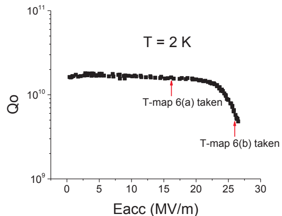
Figure 5: RF test results of the EP cavity. Field levels at which the temperature maps shown in Fig. 6 are taken are marked by arrows.
