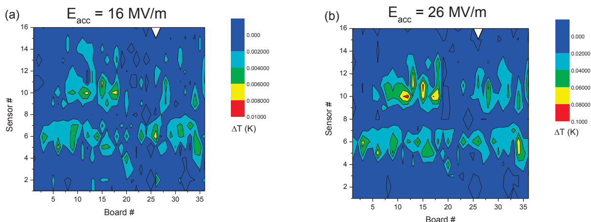
Figure 6: Temperature maps taken at (a) E_{acc} = 16 MV/m; (b) E_{acc} = 26 MV/m during the RF test shown in Fig. 5. Note a strong correlation between the heating patterns in the medium and high field Q-slope range.
