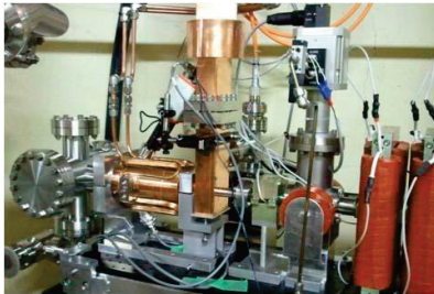
Figure 2: RF gun system installed at 3-2 section.
