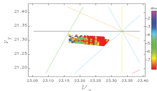
Figure 5: Tune footprint. The color reflects the tune change in terms of the tune diffusion defined in Fig. 4.
