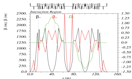
Figure 2: Optics of a complete IR in the MEIC ion ring.
