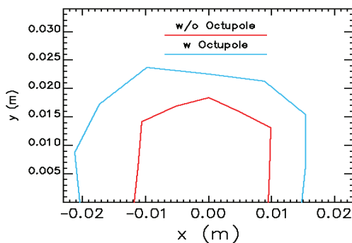
Figure 6: Dynamic aperture in the ( y - x ) space for the MEIC ion ring without (red) and with (blue) octupole minimization of the 1 st order amplitude dependent tune shift.
