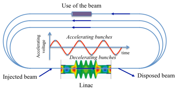
Figure 1: A sketch of a three-pass ERL.
