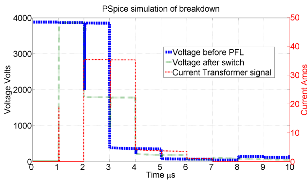
Figure 2: Breakdown simulation
