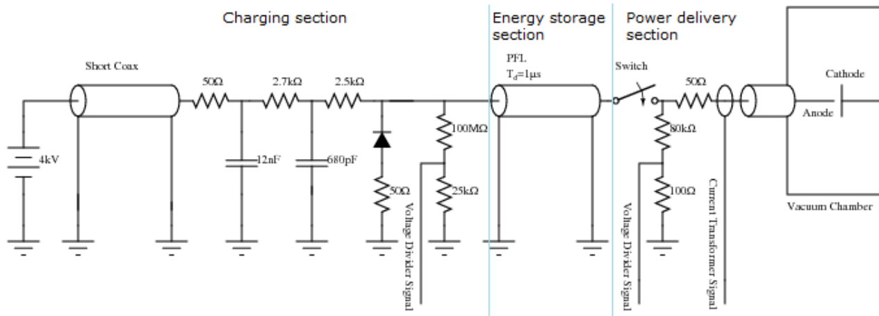
Figure 1: Circuit diagram of the new high-rep-rate CERN DC spark system. Use of coax, matched impedances and the fast switching time of the MOSFET switch allow much better insight into the turn on time of the breakdown.
