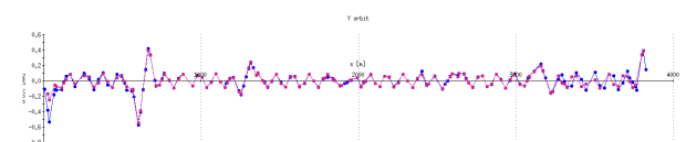
Figure 9: The vertical difference orbit (blue) vs fitted orbit (red) using range from 2000 to 2800 m and forward propagation.
