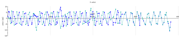
Figure 3: Measured horizontal difference orbit (blue) versus the fitted orbit by backwards propagation.
