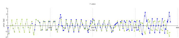
Figure 5: Measured vertical difference orbit (blue) versus the fitted orbit by forwards propagation.
