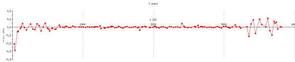
Figure 11: The difference of original difference orbit and forward propagated fit orbit.
