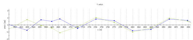
Figure 8: The region (by zooming in Fig. 7) where the fitted orbit starts to deviate from the difference orbit.
