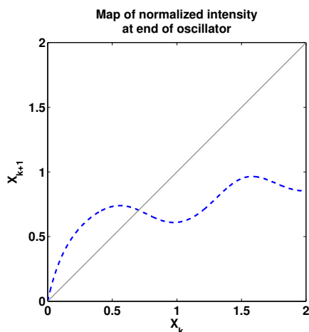
Figure 2: Normalized intensity at the end of the oscillator as a function of the normalized intensity at the end of the oscillator in the previous pass. The equilibrium point occurs at 0.70, and has a slope for the map of -0.44, indicating it is stable with damped oscillations.
