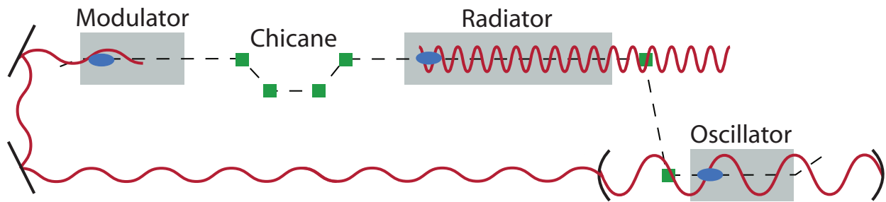
Figure 1: A schematic of a radiator-first configuration for oscillator seeding of a high gain harmonic generation FEL. Electron bunches are shown as blue ovals and the path of the radiation as wavy red lines. The power in the modulator seen by a bunch is generated in the oscillator by earlier bunches. The transfer line taking the electron beam from the radiator to the oscillator is not shown in detail because it has little effect on performance; the only requirement is that short-wavelength bunching should be suppressed.
