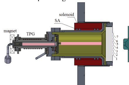
Figure 1: Drawing of the SA Plasma generator with RF TPG and plasma plate with 7 collectors opposite 7 emission apertures of 2 mm diameter ( S=3.2 \text{ mm}^2 ). Magnetic accelerator electrode is attached for producing of correct magnetic field distribution.
