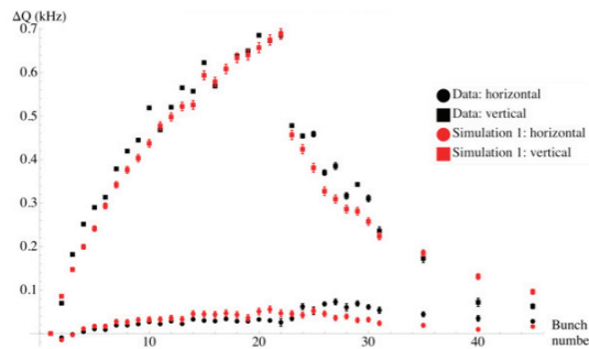
Figure 2: Tune shifts vs bunch number for a train of 20 bunches with 14 ns spacing. Witness bunches measure the decaying cloud density beyond the end of the train at 14ns intervals. Black points are data, squares are vertical and circles horizontal tune shifts. The red points are from POSINT simulations using best fit physics parameters.
