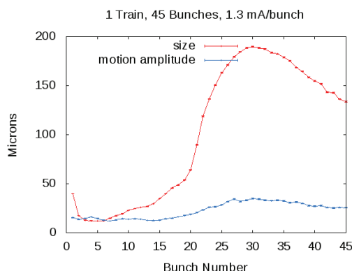
Figure 3: Vertical size (red) and centroid motion (blue) of each bunch measured with the xBSM vs bunch number in a 45 bunch train, with 2 \times 10^{10} e^+ / \text{bunch} .
