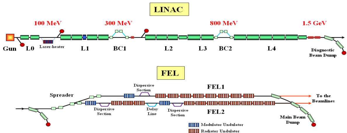
Figure 1: Layout of the FERMI@Elettra linac and Free Electron Laser (FEL).
