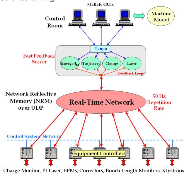
Figure 2: Fast feedback architecture.
