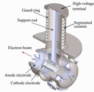
Figure 3: A schematic drawing of a 500-kV, 10-mA photocathode gun which was constructed at JAEA.
