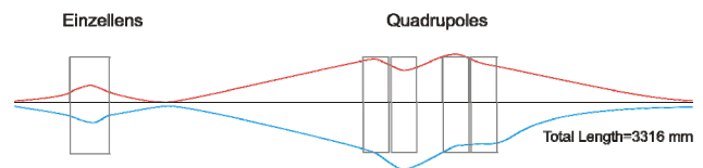
Figure 1: Overview of the injection beam line including the set of four quadrupoles.
