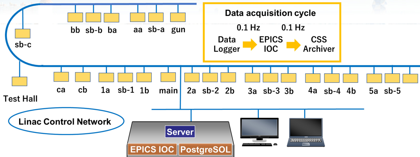
Fig. 2: Schematic layout of data acquisition software.
