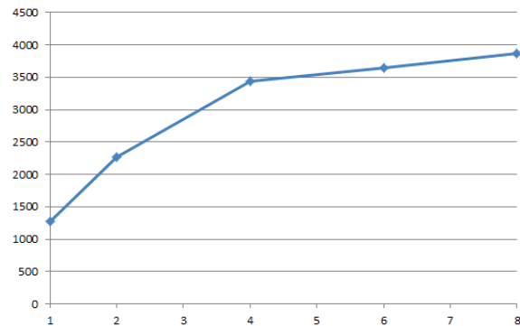
Figure 1: Performance of Graphene in a multi core environment. Number of plots per second vs number of threads.
