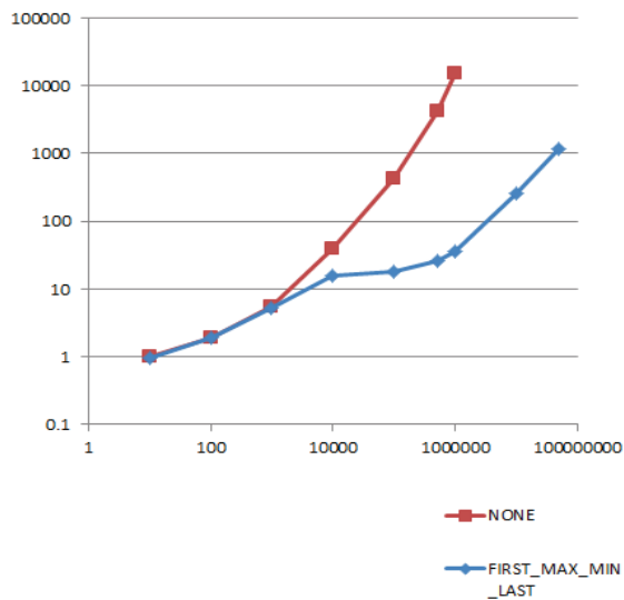
Figure 3: Comparison of the performance for producing line plots with and without data reduction. Number of points plotted vs plotting time in milliseconds.
