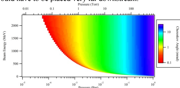
Figure 5: Cherenkov emission angle for an electron beam crossing a CO 2 gas jet.
