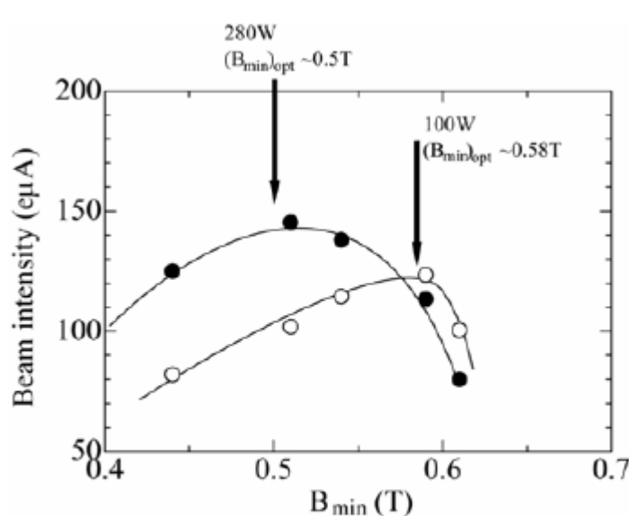
Fig 3 Beam intensity of Ar^{28+} as a function of B_{min} at the RF power of 100 and 280 W.
