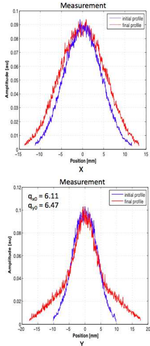
Figure 1: Beam profiles after 1 second storage of the beam in the CERN-PS. The asymmetry of the beam response is evident.
