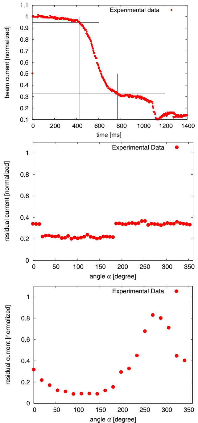
Figure 3: Top: beam survival by crossing the resonance Q_x + 2Q_y = 11 in 1 second. The survival is \sim 35\% . Center: effect of the power supply, note the discontinuity of beam survival at \alpha = 20,170 degree for a small driving term. Bottom: best compensation for \Lambda = 0.025 at \alpha = 270 degree.
