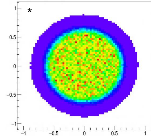
New approach: Core + Halo generation for simulations
