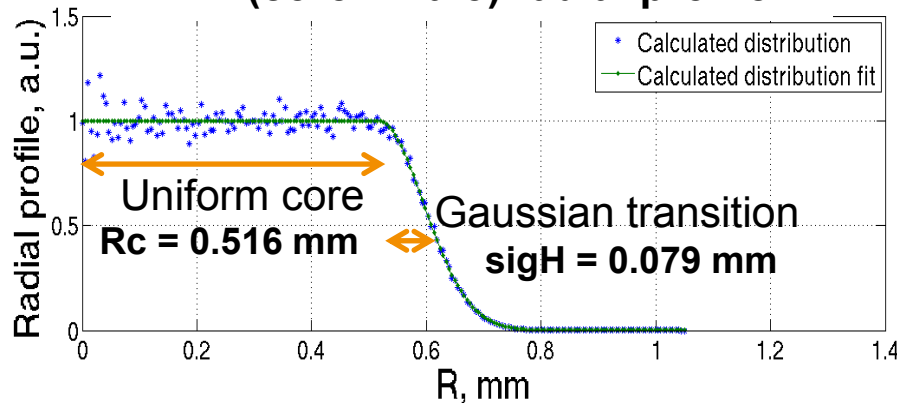
CH (core + halo) radial profile
