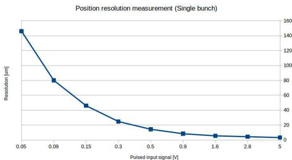
Figure 6: Single bunch measurement performance versus input signal level (0 dBFS = 5 V peak).
