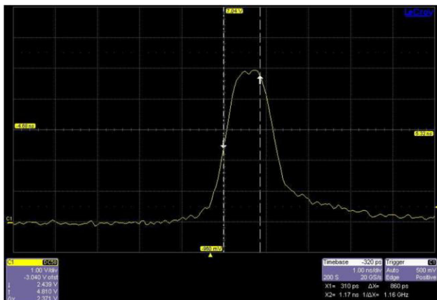
Figure 7: Input signal.
