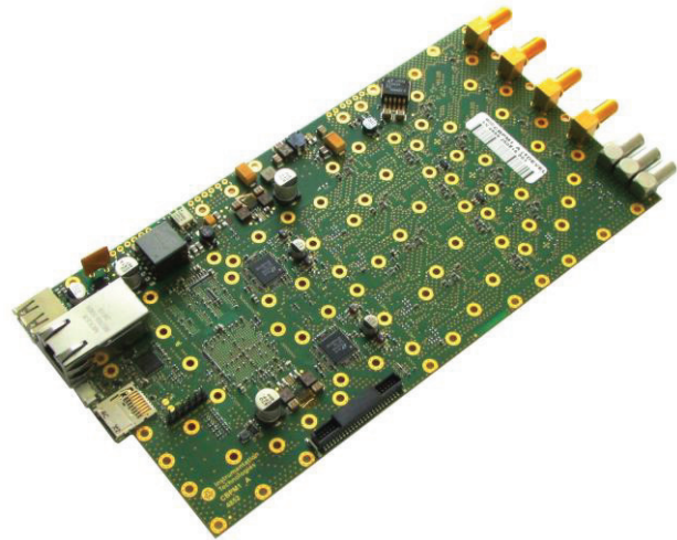
Figure 3: Libera Spark EL.
