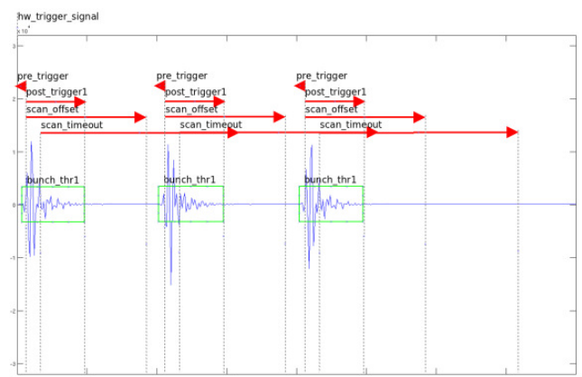
Figure 5: Macro-pulse mode.
