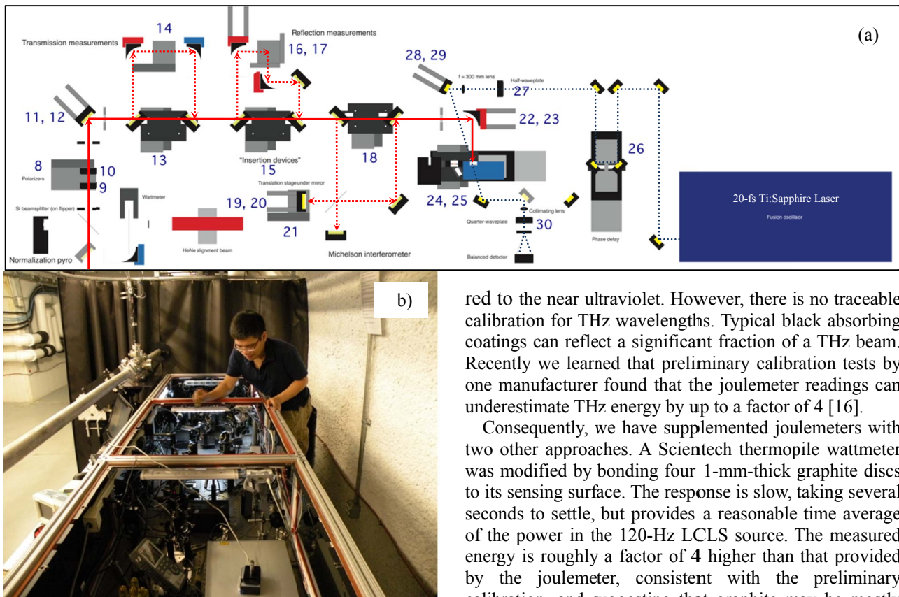
Figure 1: (a) Layout of optics on the THz table. The THz (red lines) enters at the lower left. (b) LCLS electron and x-ray beams travel through the beampipe above the optical table in the LCLS undulator hall. The cross at the far end of the table holds the actuator that inserts the THz foil, with the exit window below. The THXPP project will go on the empty table space directly below the beamline.
