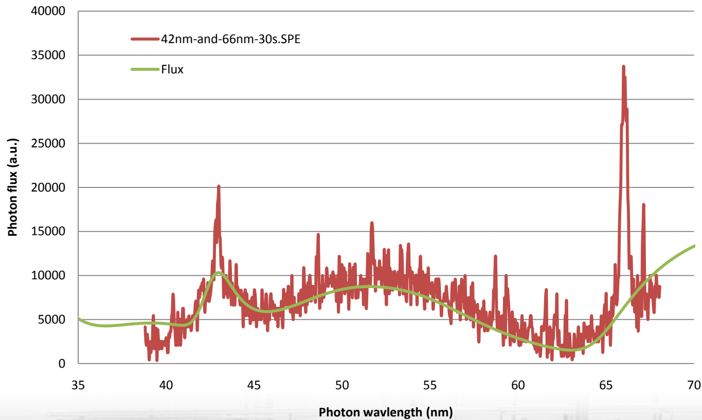
CHG undulator spectrum
