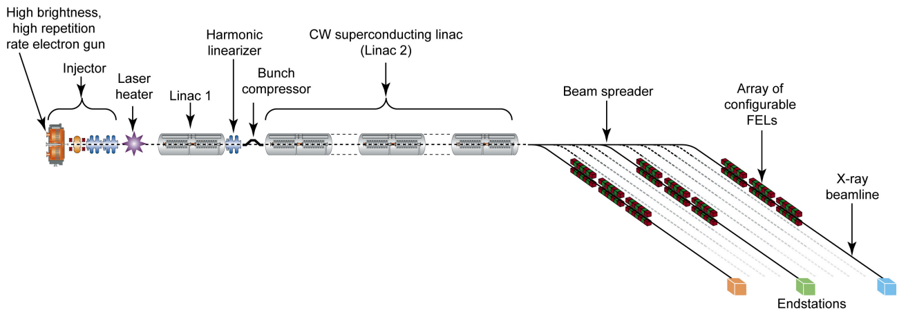
Figure 1: Schematic layout of the NGLS.
