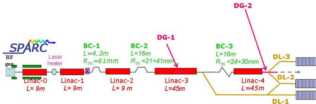
Figure 1: SPARX-FEL Layout
