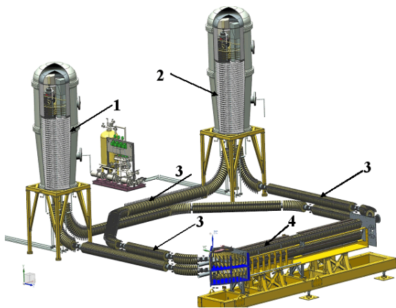
Fig.4. General view of the electron cooling system (II). 1, 2 – tanks with electron gun and acceleration tube and deceleration tube + collector, 3 – beam transportation solenoids, 4- electron cooling section
