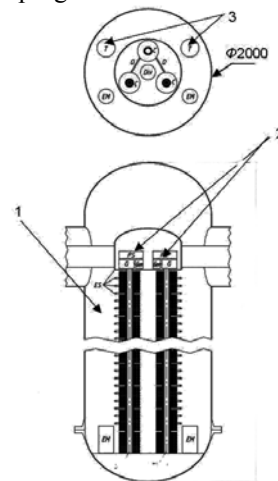
Fig.2. Design of power supply of 2.5 MV. 1 - cascade generator, 2 - gun and collector power supply, 3 - power transmitters to high potential ("shafts")
