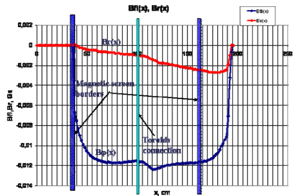
Fig.6. Magnetic field distribution on the electron beam axis near connection in the toroidal solenoids of different diameters; x-coordinate along electron trajectory
