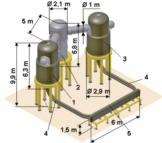
Fig.1. General view of the electron cooler. 1, 3 – the tanks with electron gun and acceleration tube and deceleration tube + collector for electron beam of opposite direction, 2 – tank with HV generator, 4 – beam transportation solenoids, 5- electron cooling section
