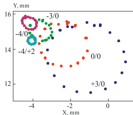
Figure 8: Larmour oscillation of the electron beam at the currents in the dipole correctors (line10-1). The numbers near curves are currents in the horizontal and vertical correctors. The electron energy is 1 MeV. The electron angle without correction is 40 mrad. The magnetic field in BPM region is 950 G.
