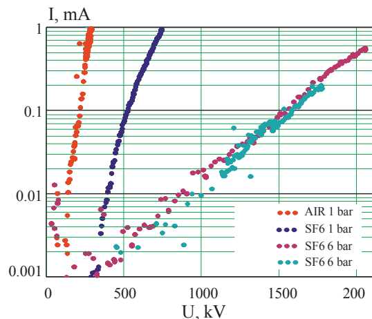
Figure 2: Corona current versus high voltage.
