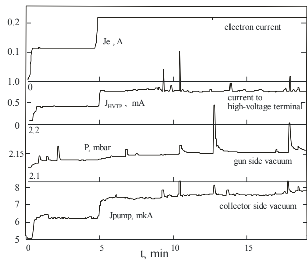
Figure 11: Electron current, leakage current to the high-voltage terminal, vacuum condition in the gun and collector sides versus time. Fragment of training of a new regime.
