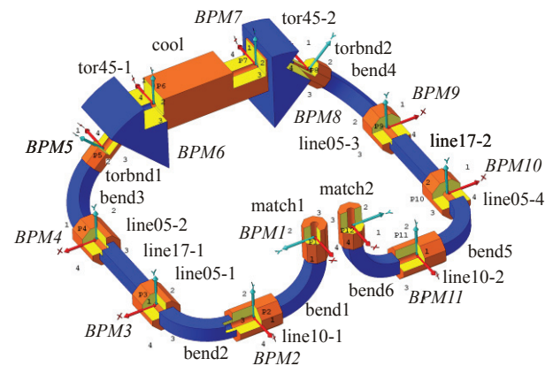
Figure 7: Location of the BPM (marked by arrows) and magnetic elements of COSY cooler.
