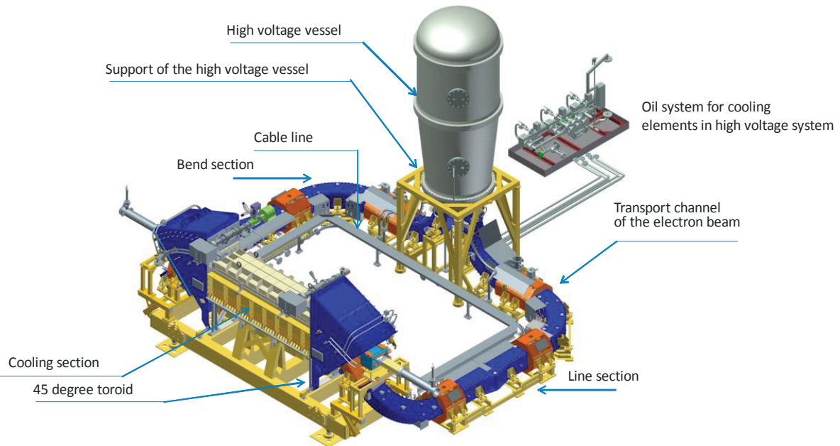
Figure 1: 3D design of 2 MeV COSY cooler.
