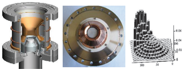
Figure 6: Design of the electron gun and 4-sectors control electrode. The right picture shows the distribution of the electron current when the control voltage is applied to the single sector.
