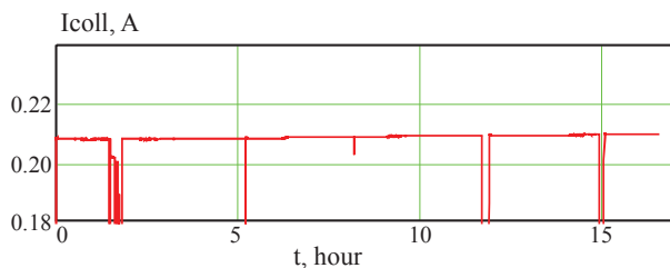
Figure 10: Collector electron current versus time. Fragment of 24 hours of running the electron beam.
