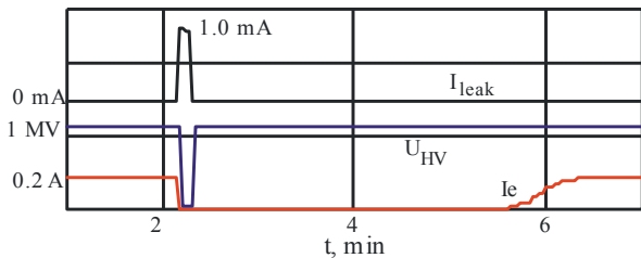
Figure 3: Collector current, voltage of the electrostatic generator and leakage current in time of the recuperation breakdown.
