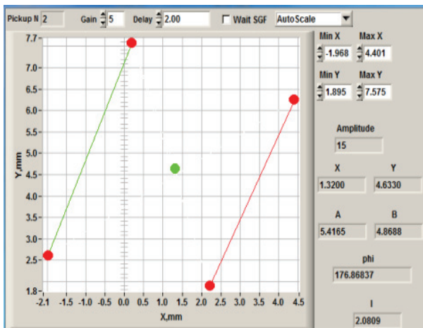
Figure 5: Measure of the electron beam position and the beam shape with 4-sectors electron gun.
