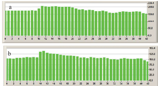
Figure 4: Distribution of auxiliary voltage along the accelerating column. The sections 10-42 correspond to column; the sections 0-9 are high-voltage terminal. The variant (a) is no-load operation of the cascade transformer, the variant (b) is operation at the nominal current in high-voltage sections (2.5 A) and the electron current 0.5 A in the collector.
