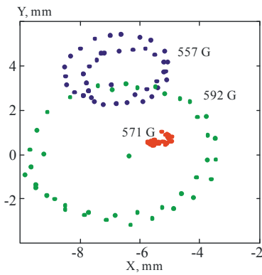
Figure 9: Radii of Larmor rotation at the different value of the longitudinal magnetic field in the bend magnets. The electron energy is 500 keV.
