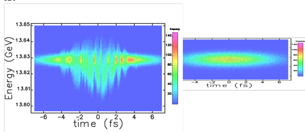
Figure 4: Beam simulation result at the spectrometer screen with the FEL on (left) and FEL off (right).
