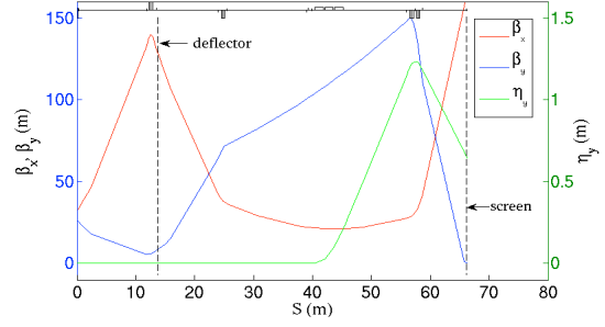
Figure 3: Optics from the deflector to the spectrometer screen.
