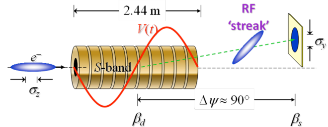
Figure 1: Principle of operation of the TCAV.
