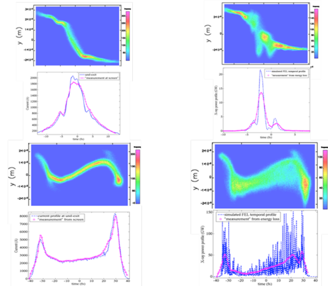
Figure 5: Reconstructed beam current profile (left) and photon intensity (right) for soft x-ray operation (top) and hard x-rays (bottom) from reference [3].
