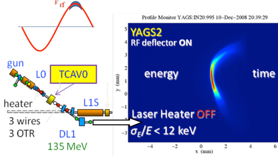
Figure 2: Time-energy correlation measurement.
