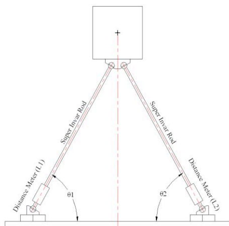
Figure 5: BPM position monitor concept.
