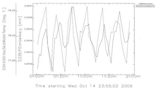
Figure 3: Sector 34 IDVC BPM readback and chamber water temperature variation over a two-hour period.
