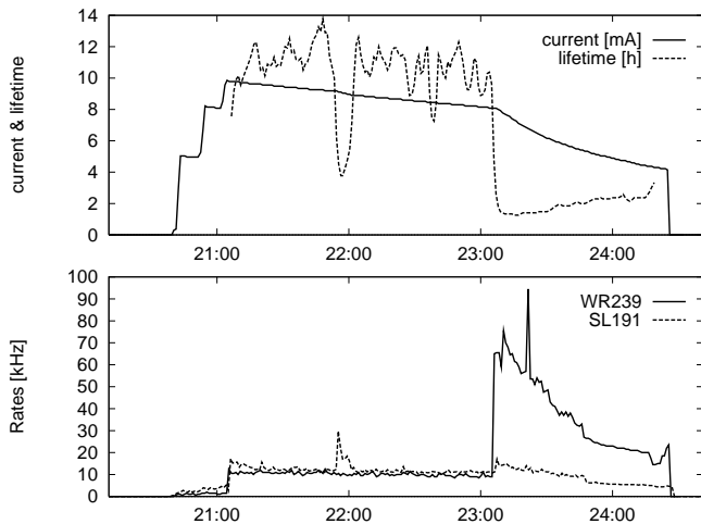
Figure 6. Lifetime reduction events correlate well with losses seen in the HERA electron loss monitors. In the above example from 11 Oct 1994 the brief disruption of the lifetime and current at time 21:55 is seen in loss monitor SL191, and the irreversible disruption at 23:05 is seen in monitor WR239.
