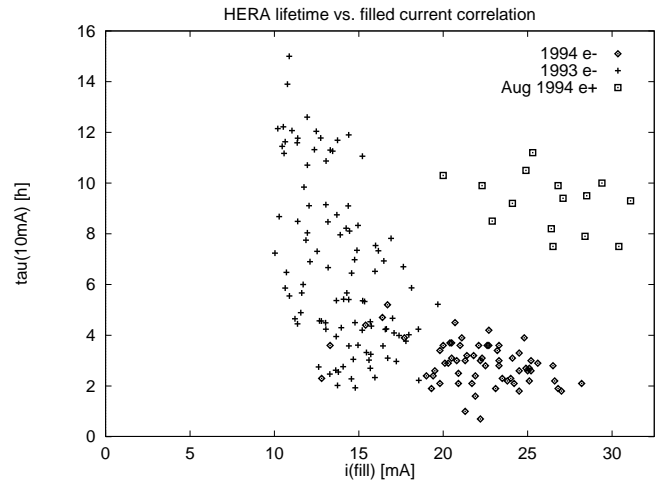
Figure 5. The lifetime in hours at beam current 10mA is plotted against the filled current for HERA electron runs in 1993 and 1994, and for positron runs in August 1994.
