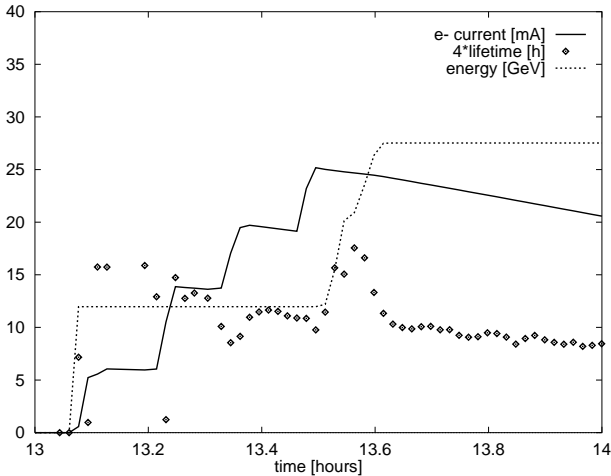
Figure 3. An example of the HERA electron beam lifetime development during the ramp from energy 12GeV to 27GeV for electrons. The current, lifetime and energy are shown against the time in hours. The electron beam lifetime tends to peak during the ramp and then drop.
