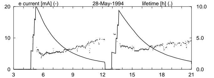
Figure 4. The electron lifetime frequently decreases gradually at the beginning of a run.
