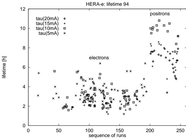
Figure 2. HERA electron and positron beam lifetimes in from March to August 1994 at current values i = 5, 10, 15, and 20 mA. The run for run sequence is shown.
