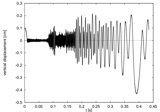
Figure 7. A simulation of the expulsion of a trapped 1\mu\text{m} dust particle from the HERA electron beam by sweeping a transverse beam kick through kHz frequencies.
