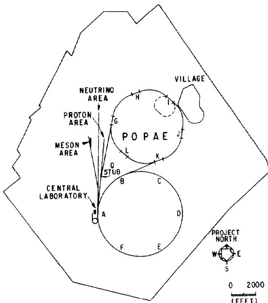
Fig. 2. Location of POPAE on the Fermilab site. The dashed ring shows a possible future location of a 20-GeV electron storage ring for ep collisions.
