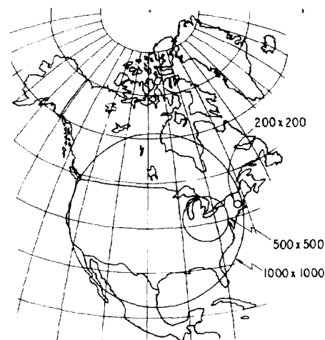
Fig. 1. Size of fixed-target accelerators (with 40 kG dipoles) to achieve the same center-of-mass energy as proton-proton storage rings of the energies indicated (GeV).
