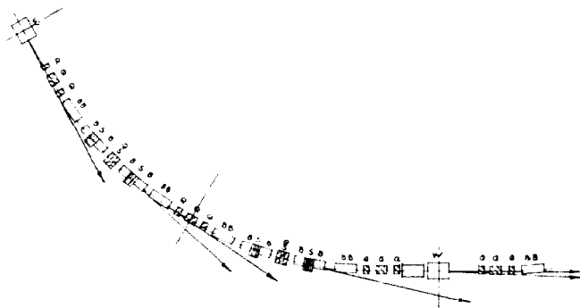
Fig. 2. Schematic of one superperiod.
