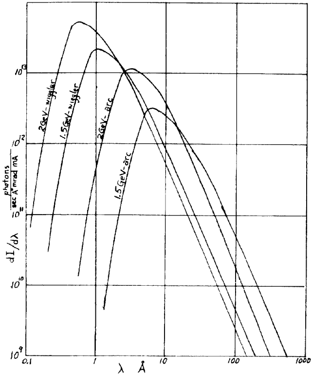
Fig. 1. Synchrotron radiation spectra.
