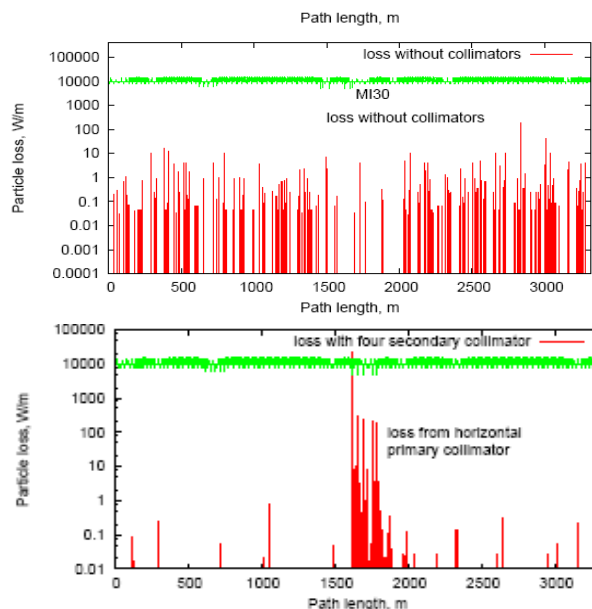
Figure 5: Power loss distribution across Main Injector without (top) and with collimators (bottom) .
