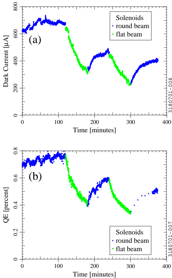
Figure 2. Measurements of (a) dark current and (b) QE as a function of time, switching between round and flat beam solenoid settings. The RF pulse length was 80 \mu s.
