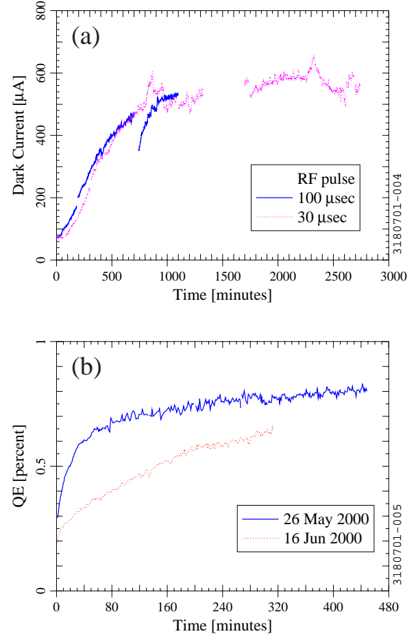
Figure 1. Measurements of (a) dark current and (b) quantum efficiency as a function of time with round beam solenoid settings. A 22 \mu\text{s} RF pulse was used for (b).
