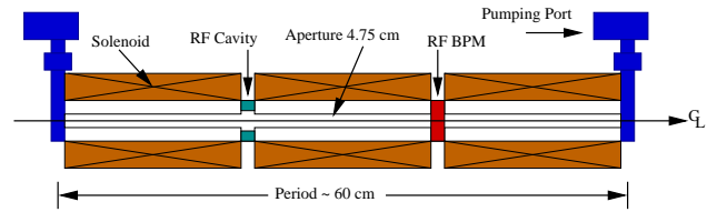
Figure 1: Minimum beamline configuration.
