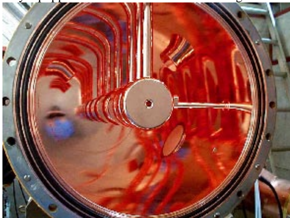
Figure 1: DTL cavity and drift-tubes.
