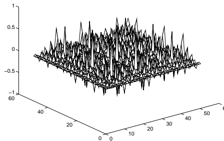
Figure 2: The solution via multiscales.
