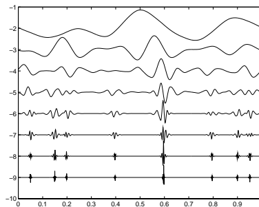
Figure 1: Multiscale/eigenmode decomposition.
