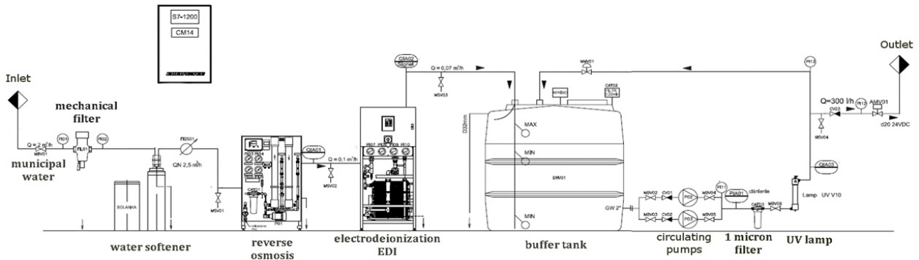
Figure 4: Water treatment plant.
