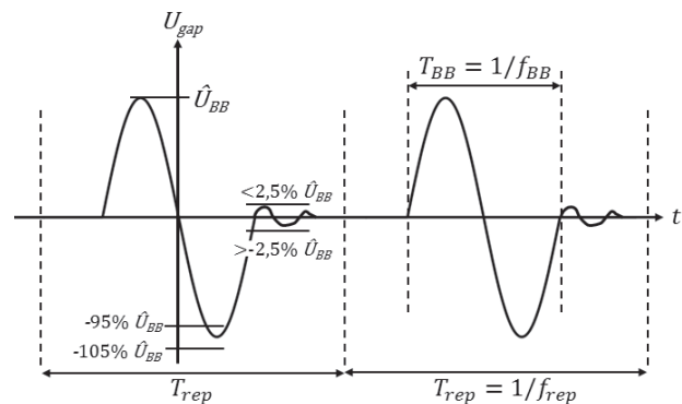
Figure 1: Desired output gap voltage.
