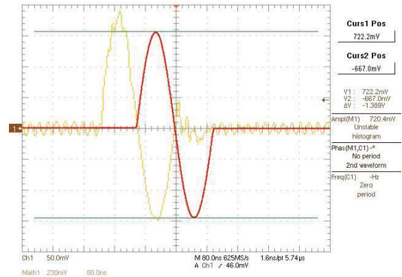
Figure 4: Measured input and output signal in the linear region ( \hat{U} = 520 V).
