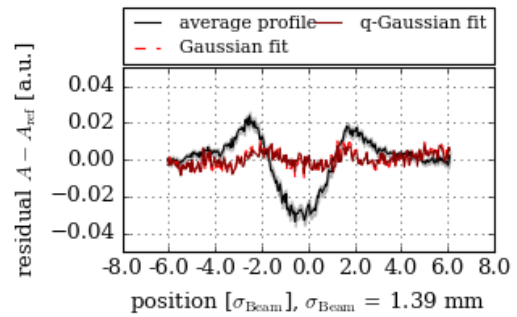
Figure 3: Residual defined as profile after excitation ( A_{\max} = 96 nrad) minus profile before excitation ( A_{\max} = 0 ) for excitation 10 th turn V. A clear depletion of the center of the distribution and increase in the middle is visible. The red lines are the deviation from the Gaussian and q-Gaussian fit indicating that the distribution also becomes slightly non-Gaussian.
