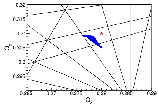
Figure 3: Detuning with amplitude up to 7 beam \sigma driven by the multipole errors Table 1 of Ref. [1], where b_{3S} has been set to 7 unit and corrected with spool pieces (for the 60 seeds used in DA simulations). The lines show resonances up to the 9 th order.
