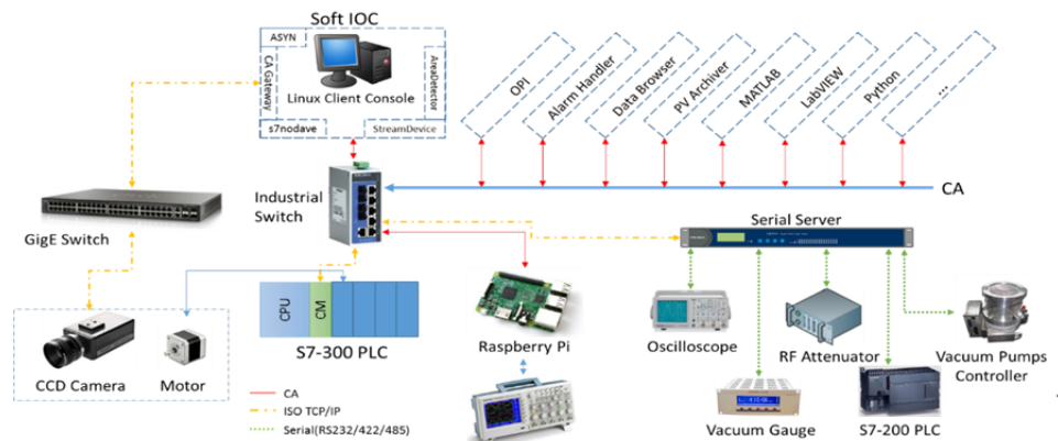
Figure 1: layout of IPM e-Linac control system network architecture.
