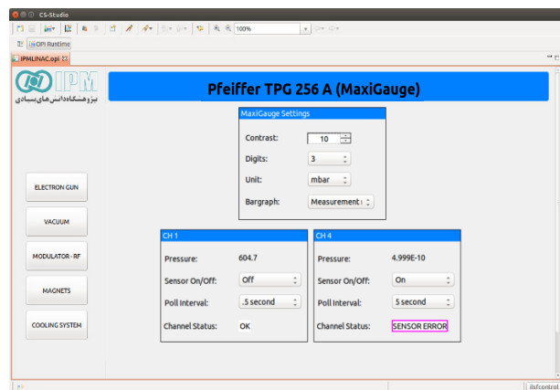
Figure 3: Vacuum setting operator screen.
