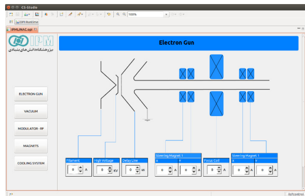
Figure 2: Electron gun operator screen.
