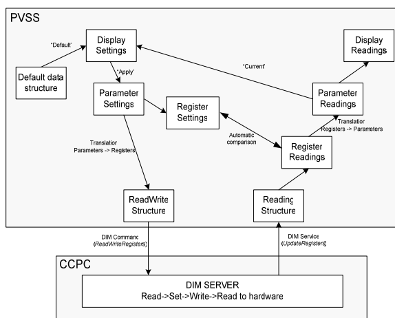
Figure 4: Flow chart of the register control.
