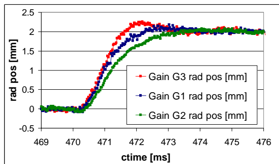
Figure 5: Radial loop response to a position step for different gain values.
