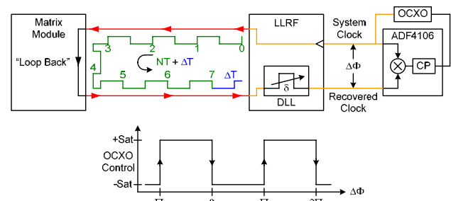
Figure 5: Eliminating the fractional cycle with the DLL.
