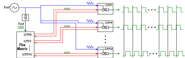
Figure 4: Locking Fref to Pref. Clock phases are fixed.
