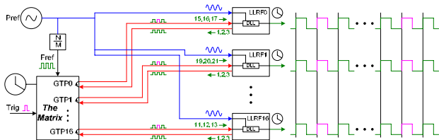
Figure 6: Setting the time and sending triggers.
