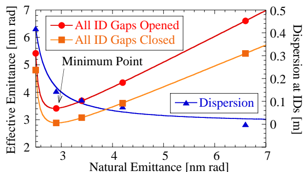
Figure 1: Effective emittance at SPring-8 storage ring.
