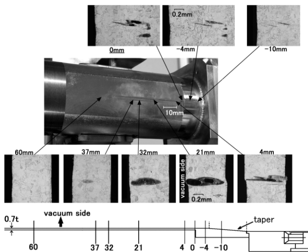
Figure 2: Injection chamber damaged by electron beam.
