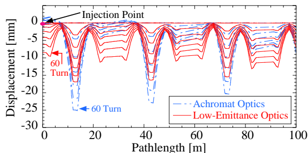
Figure 3: Calculated horizontal beam trajectories at 1, 10, 20, 30, 40, 50 and 60 turns after cutting off the RF power.
