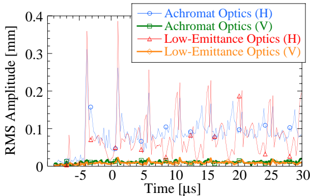
Figure 4: Oscillation of a stored beam at beam injection. Revolution period is 4.8\mu\text{s} .
