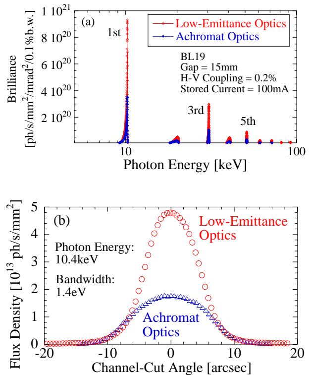
Figure 5: Comparison of brilliance and flux density. (a) Calculated brilliance and (b) observed flux density in BL19LXU long-undulator beamline.
