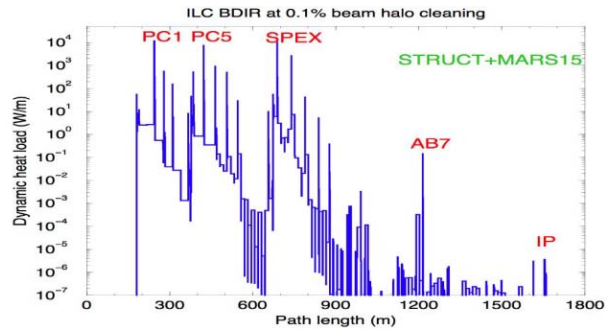
Figure 4: Power dissipation in the 20 mrad BDS using MARS15.
