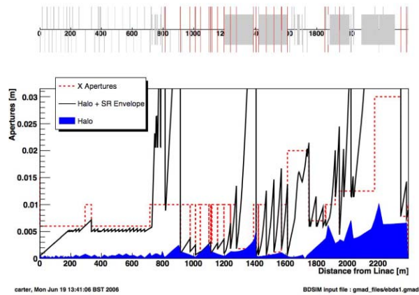
Figure 5: Beam envelope of the halo (shaded region) and the collimated SR (solid line) in the 20 mrad BDS. Horizontal aperture of elements is also plotted (dashed line).
