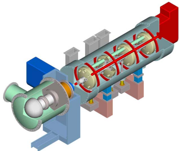
Figure 1. Engineering model of the DC gun and SRF cryomodule high-power CW injector.
