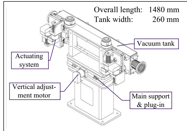
Figure 1: Design view of an LHC secondary collimator.
