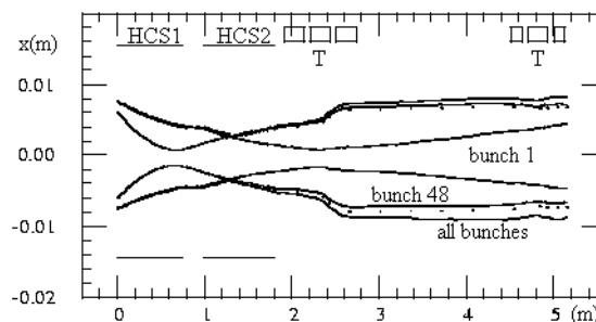
Figure 5: Envelope with transverse wake-field for bunches 1 and 48, all bunches, and with no wake-field (structures transverse displacement is 0.5 mm)
