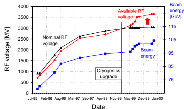
Figure 1: Evolution of beam energy, nominal RF voltage (design gradient) and available RF voltage [2].
