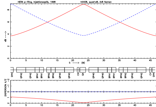
Figure 4: Beam optics in the FODO section of HERA-p
